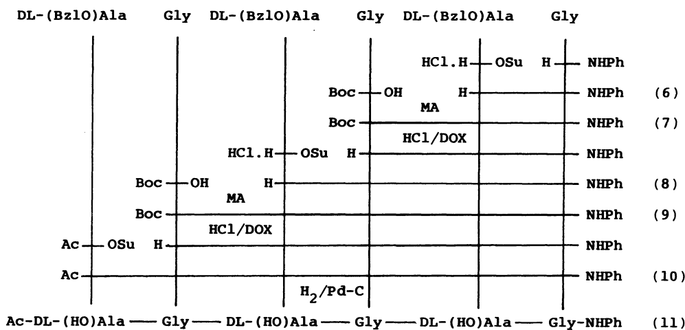
Fig. 2. Synthesis of an N -hydroxy hexapeptide (11) via N -benzyloxy peptides (6—10): BzlO stands for PhCH 2 O and DOX for dioxane. Acylation by the mixed anhydride procedure was repeated 3 times.
